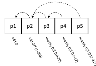
Figure 3: A repository state showing patch dependencies.
