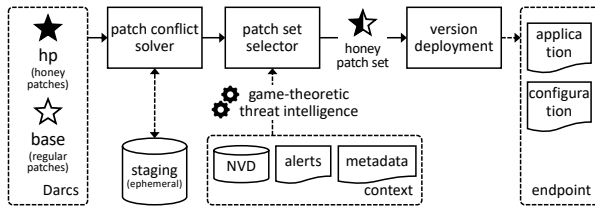
Figure 2: An overview of QUICKSAND.
